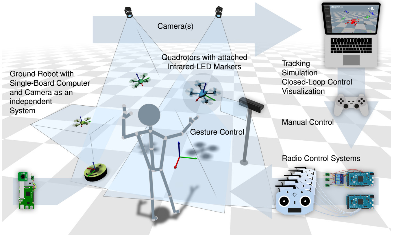
Fig. 1: Overview of ICARUS : After pose estimation of the individual quadrotors based on optical tracking the control variables are determined and sent via different radio control systems to the quadrotors.
