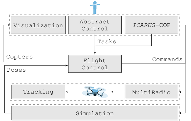
Fig. 3: The software architecture of ICARUS .
